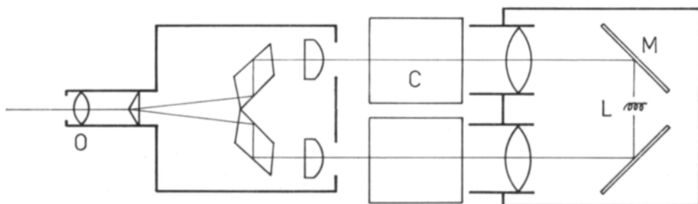
Fig. 1. Schematic picture of the comparator. L lamp, M mirror, C optical cell, O ocular.
