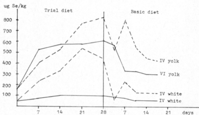
Fig. 2. Selenium content ( \mu\text{g}/\text{kg} dry matter) of eggs in trial groups IV and VI during the trial and after transfer back to the basic diet.
