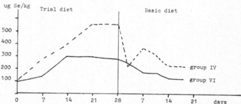
Fig. 3. Selenium content of egg yolk and white in trial groups IV and VI during the trial and basic diet period.
