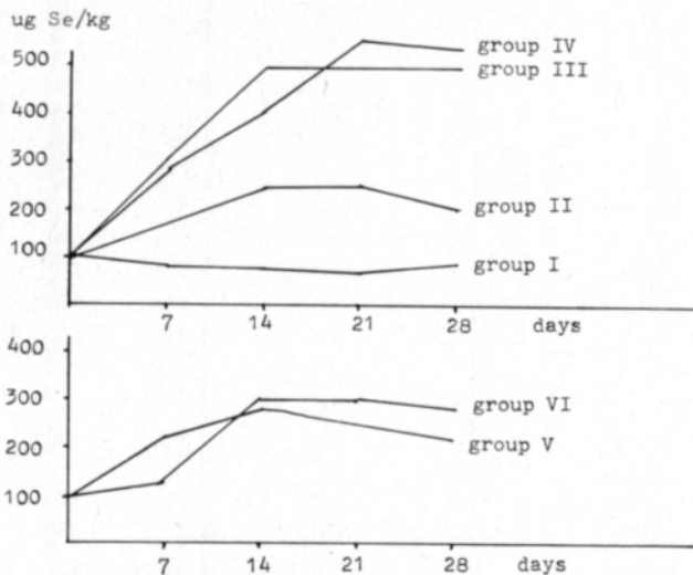
Fig. 1. Effect of selenium content of feed on that of eggs in different trial groups during the trial.
