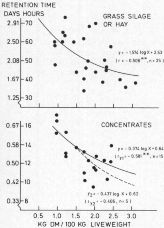
Figure 11. Ruminal retention times of hay, grass silage and concentrates when the feeding level of an animal and the ratio of roughage to concentrate ( y_1 , 70:30, y_2 , 50:50) in the diet varied ( y and x as in Figure 10). Material is based on data collected from the literature, for references, see Appendix 4.
