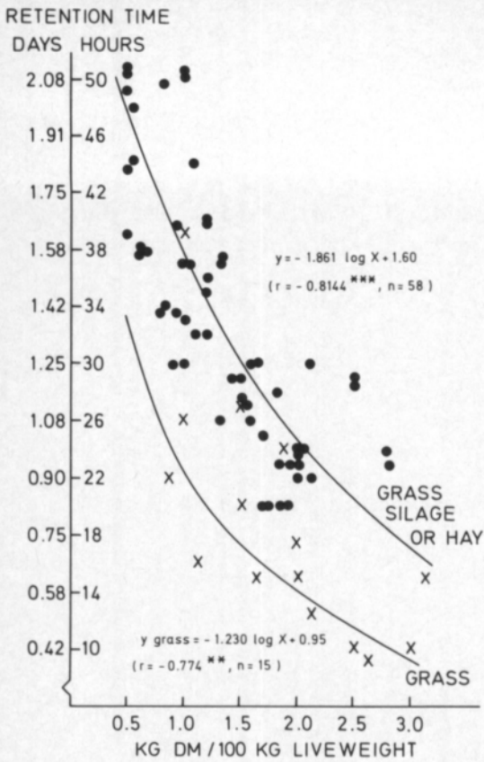
Figure 10. Ruminal retention times of hay, grass silage, and grass at different feeding levels of an animal on roughage diets ( y = retention time, days, x = kg DM/100 kg liveweight). Material is based on data collected from the literature, for references, see Appendix 4.
