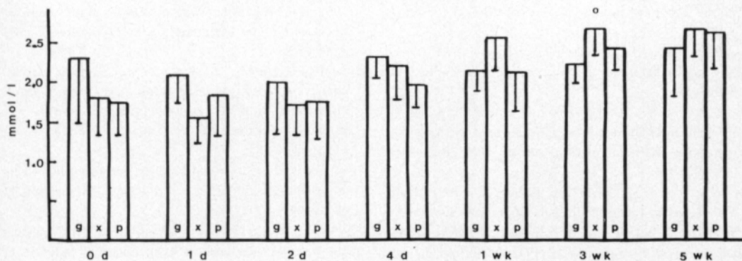
Fig. 4. Plasma P_i (means and standard deviations) in different groups from birth to the age of 5 weeks. g = glucose, x = xylitol and p = polyol molasses group. \circ The xylitol group differs from the glucose group ( P < 0.01 ).
