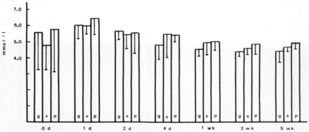
Fig. 2. Plasma glucose (means and standard deviations) in different groups from birth to the age of 5 weeks. g = glucose, x = xylitol and p = polyol molasses group.
