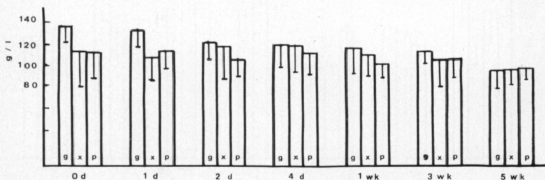
Fig. 1. Haemoglobin (means and standard deviations) in different groups from birth to the age of 5 weeks. g = glucose, x = xylitol and p = polyol molasses group.
