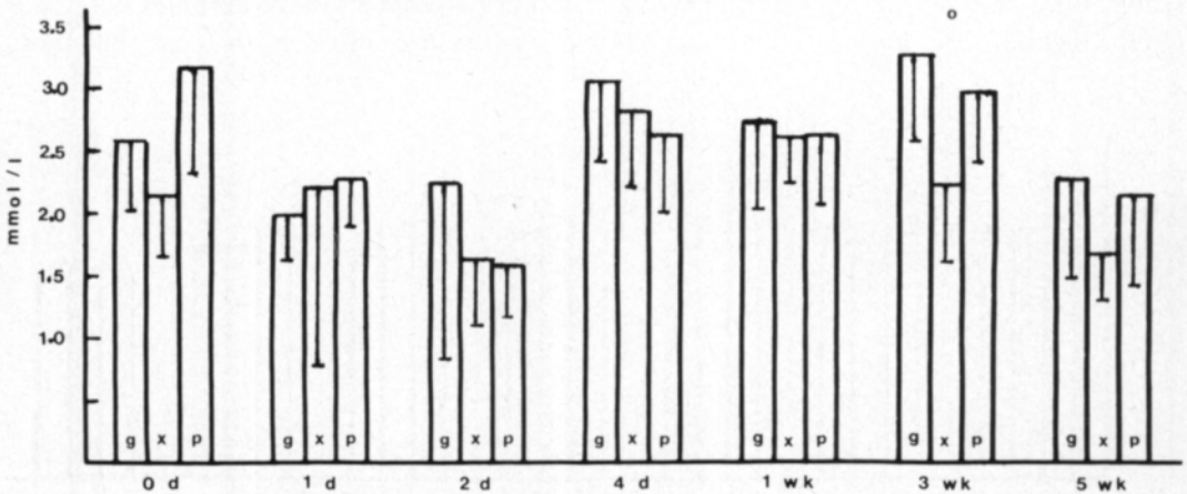
Fig. 3. Plasma urea-N (means and standard deviations) in different groups from birth to the age of 5 weeks. g = glucose, x = xylitol and p = polyol molasses group. \circ The xylitol group differs from the glucose group ( P < 0.05 ).
