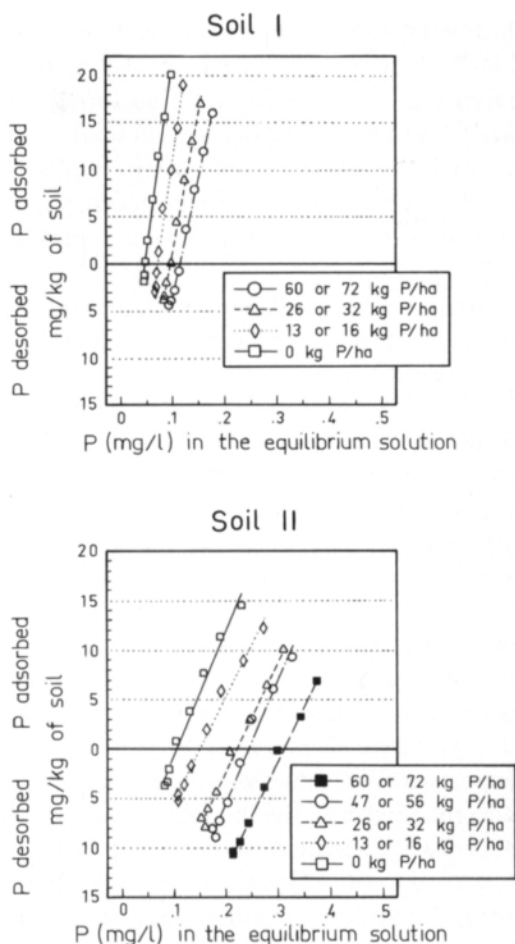
Fig. 2. Type B isotherms. Relationship between P adsorption or desorption (y) and the P concentration in the equilibrium solution (x) after adding P to subsamples of two soils (I and II) into which different rates of P had been applied annually.
