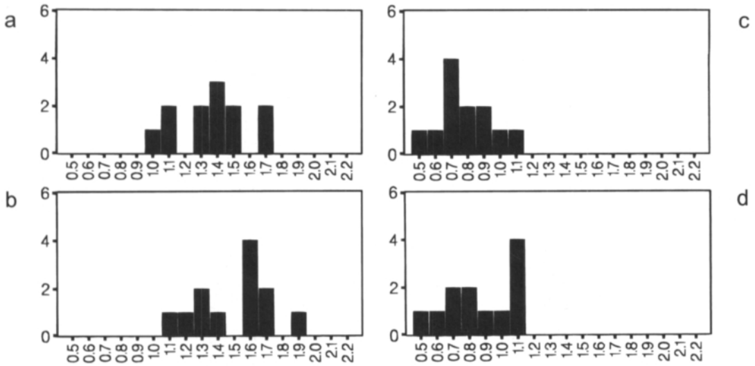
Fig. 3. Progeny of BS 06-4/2*Adorra. High-activity lines of \beta -amylase in (a) and (b).
