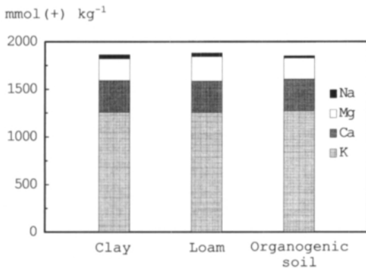
Fig. 3. Na, K, Ca and Mg concentrations of timothy (mmol of charge kg^{-1} ) in the first harvest. The plants received similar Na and K fertilization ( 200 \text{ mg dm}^{-3} , treatment Na_1K_2 ).
