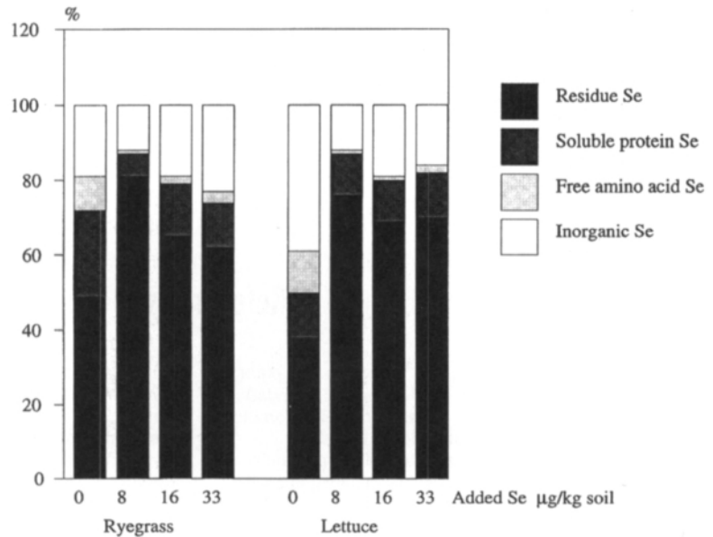
Fig. 1. The relative distribution of various Se-fractions.
