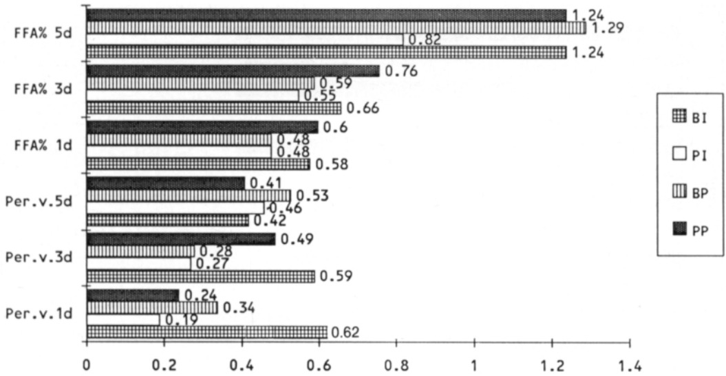
Fig. 1. Peroxide value (milliequivalents of oxygen/kg, meq O/kg) and free fatty acid (FFA %) during storage at +4°C. The test cuts BI (MDB) and PI (MDP) were recovered using the Inject Star deboner, BP (MDB) and PP (MDP) using the Poss deboner. Mean values of three replicates analysed in duplicate. Standard deviations \leq 0.4 .
