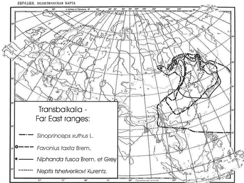
Fig. 7. Examples of Transbaikalia - Far East ranges.
