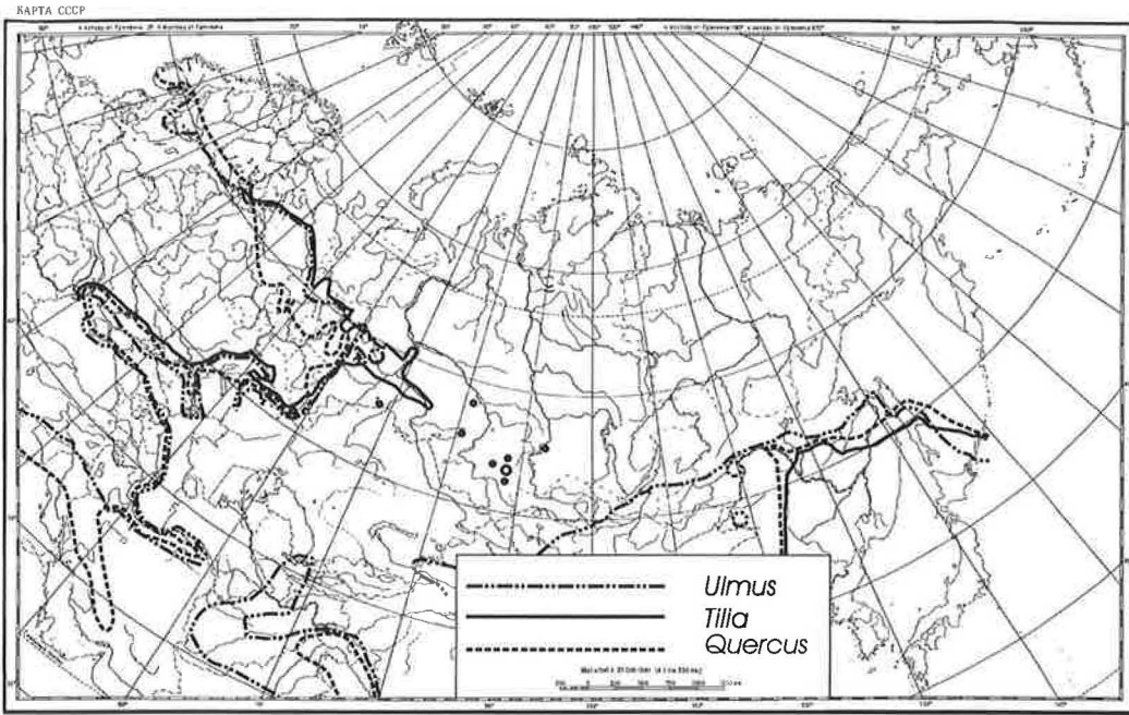
Fig. 1. Ranges of the broad-leaved tree genera present in Siberia (according to Khlonov, 1965; Gorchakovskii, 1968; Polozhii, Krapivkina, 1985; Krasnoborov, 1992, Velichko, 1993, and others).
