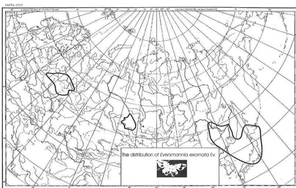
Fig. 3. Examples of Europe - West Siberia - Far East disjunctive ranges.
