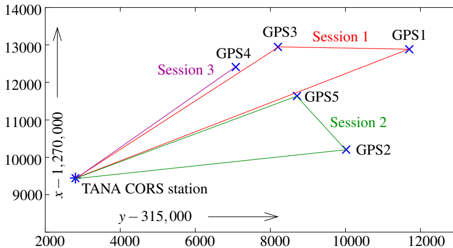
Figure 3. The GNSS network measured. Co-ordinates x, y in the Adindan UTM projection zone 37N, units: m.
