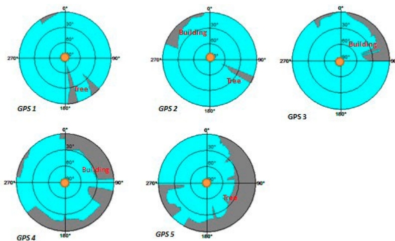
Figure 2. Obstacle sky plots of the checkpoint locations, generated by Trimble planning software.
